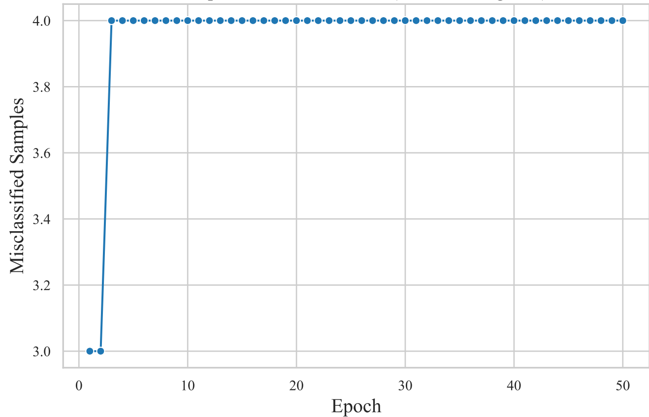
Perceptron Trained on XOR (Non-Convergence)
